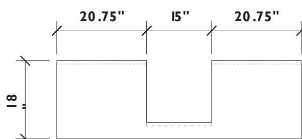
WALL Z-CLIP
